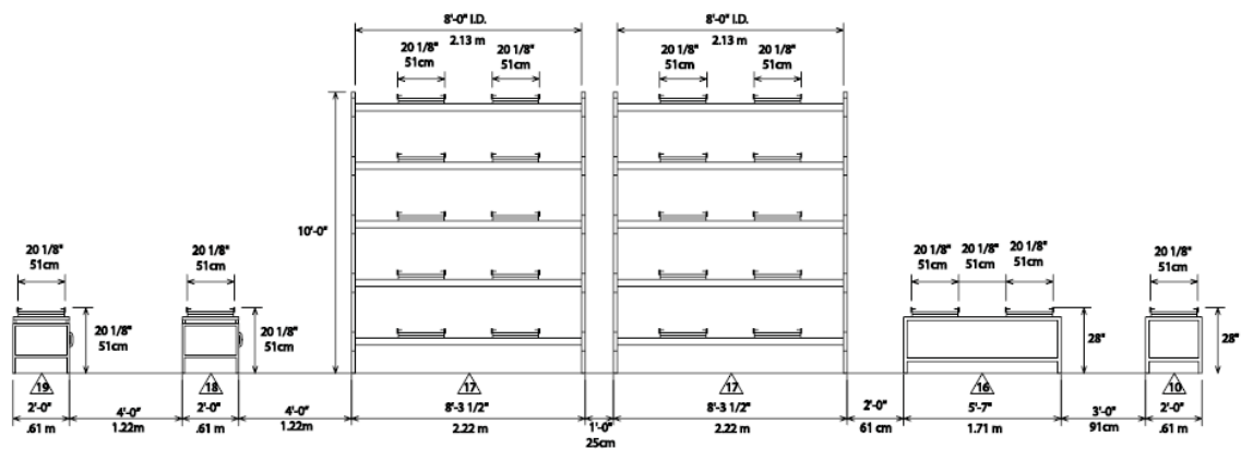
ELEVATION VIEW B-B
